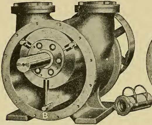
FIG. 7. END VIEW SHOWING INTERNAL CONSTRUCTION OF DURECO POSITIVE PRESSURE BLOWER
